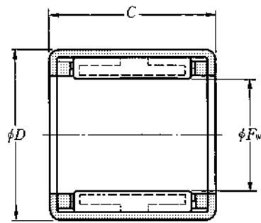
Type HF
