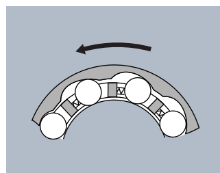
Fig. 1 One-way clutch in engagement
