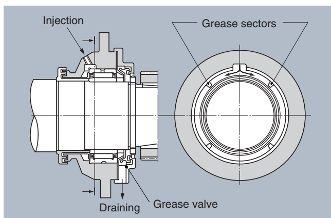
Fig. 9.1 An example of bearing unit with grease sector and grease valve
