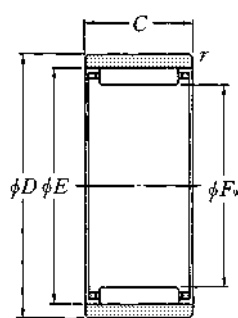
Type RNAO
