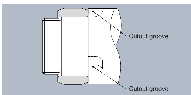
Fig. 8.4 Cutout groove for inner ring extraction
