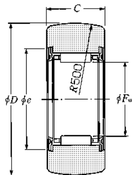
RNA22··LL type
