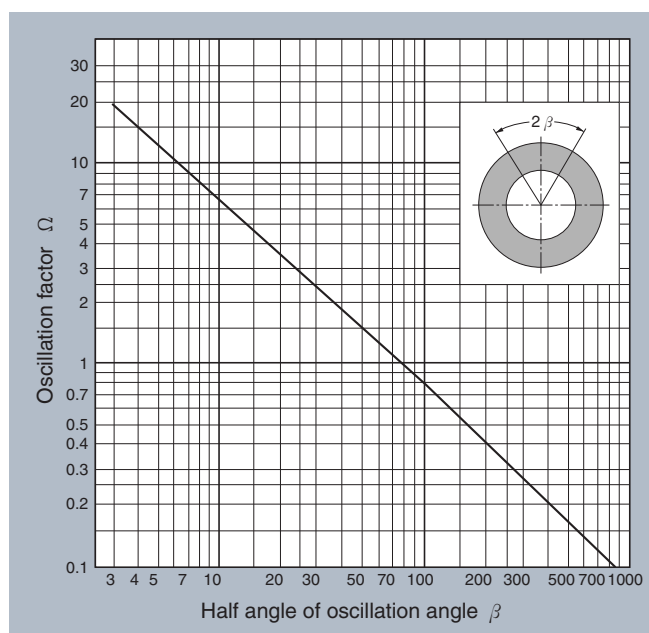
Fig. 2.3 Relationship of oscillation angle \beta to factor \Omega
