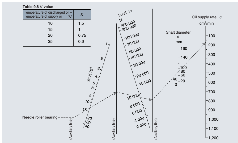
Fig. 9.6 Chart for determining oil supply rate
