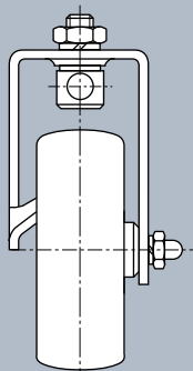
Fig. 2 Tension pulley with holder
