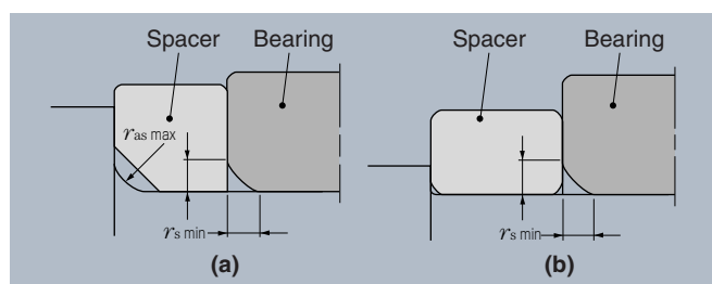
Fig. 8.11 Spacer applications
