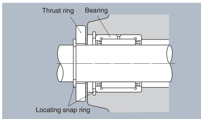
Fig. 8.2 Bearing fixing in axial direction
