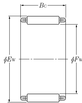
Type KJ··S
