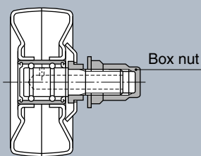
Fig. 3 Double-row bearing type tension pulley
