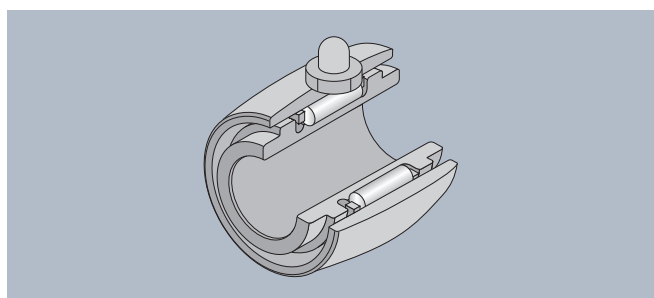
Fig.3 Type FRIS
