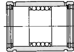
Type KD··LL (With seal)
