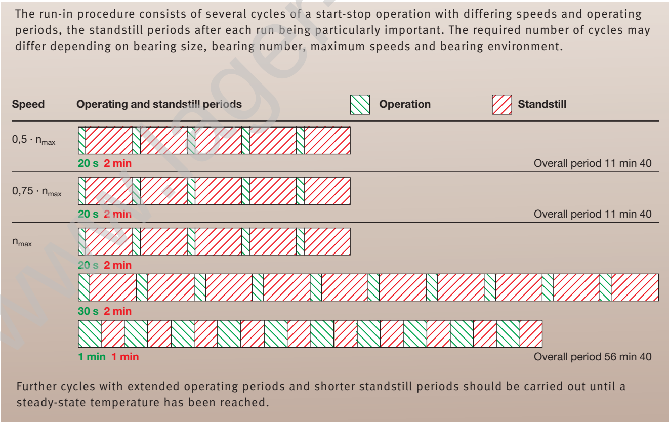
6: Recommendations for grease distribution runs of open and sealed spindle bearings
