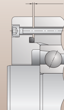
2: Recommended adjustment of face covers
