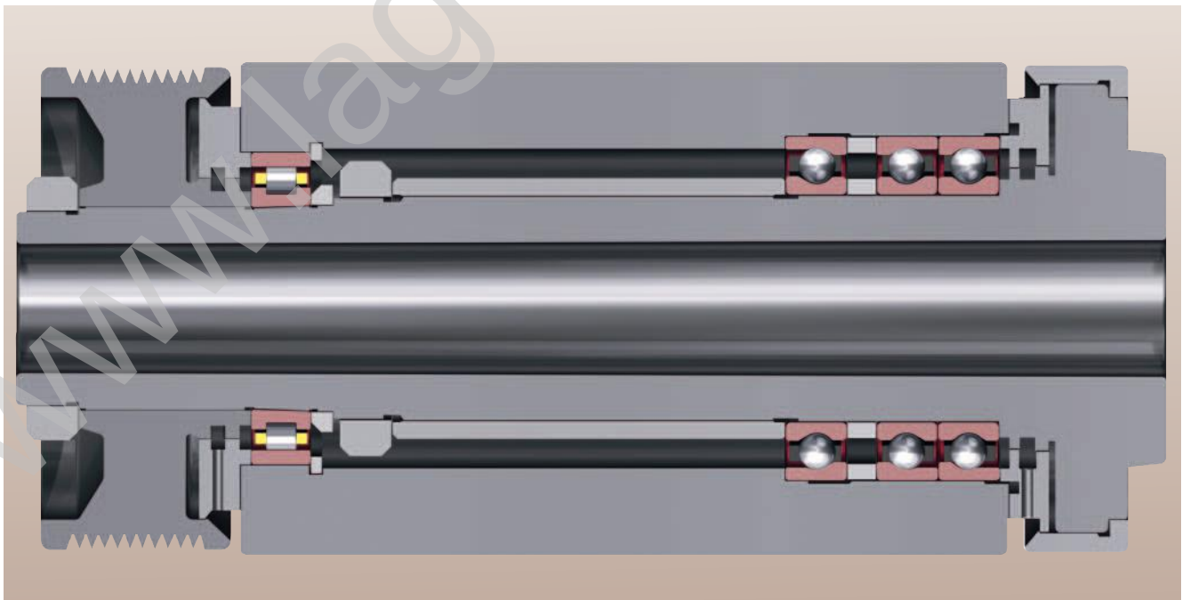
8: Turning spindle
