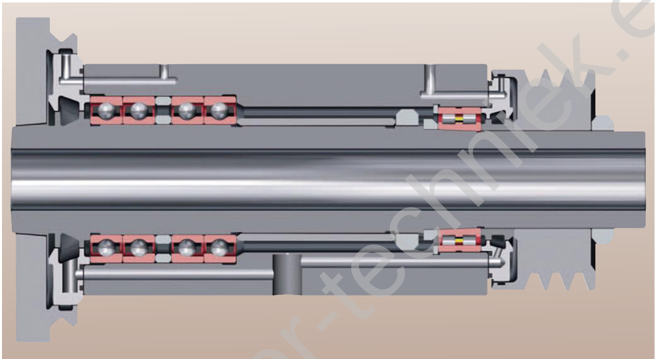
11: Grinding spindle
