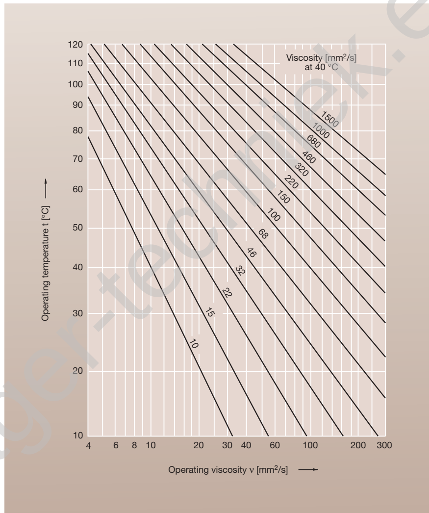
2: V-T diagram
