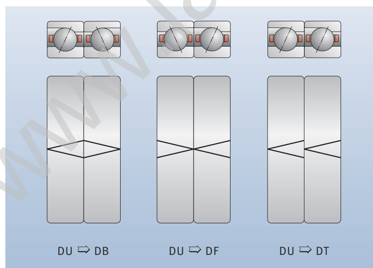
1: Installation possibilities of a DU set
